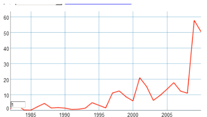
Figure 1. Temporal trends in total catch (tonnes, retained and discards) of mahi (common dolphinfish) combined, eastern Pacific Ocean, 1982 to 2010, based on catch from purse seine, longline and other fleets operating in the eastern Pacific Ocean. Catches for 2010 are provisional (IATTC, 2012).
